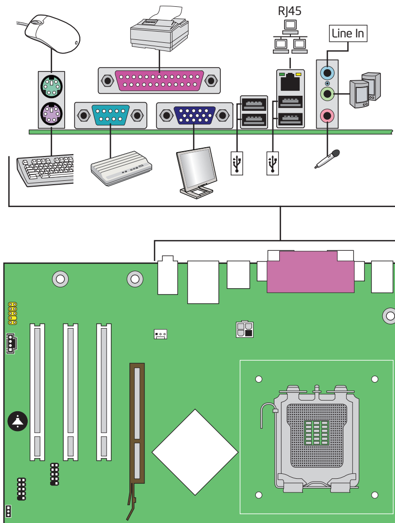
Figure 25. Back Panel Connectors
